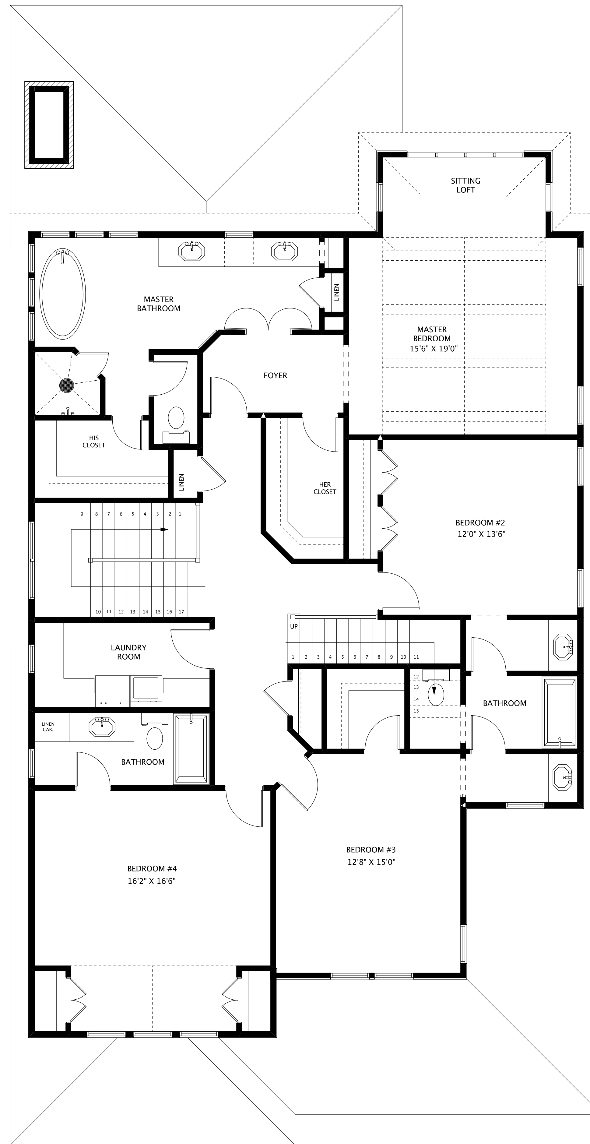
SECOND FLOOR DETAIL CONSTRUCTION SHEET
